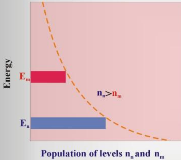
a) Boltzmann distribution; thermal equilibrium
