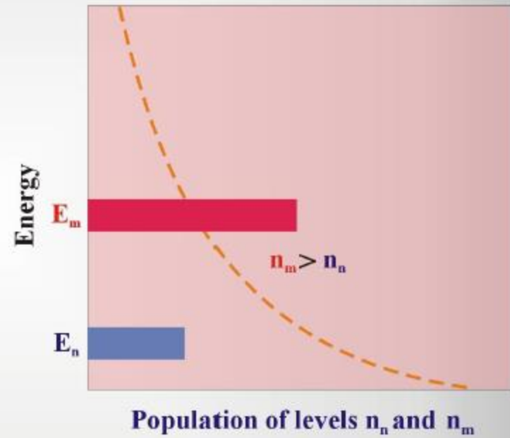
b) population inversion
